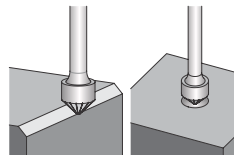
Conical counterbore shape 90°
